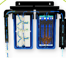
CROSS-SECTION VIEW OF WATER FILTRATION SYSTEM
